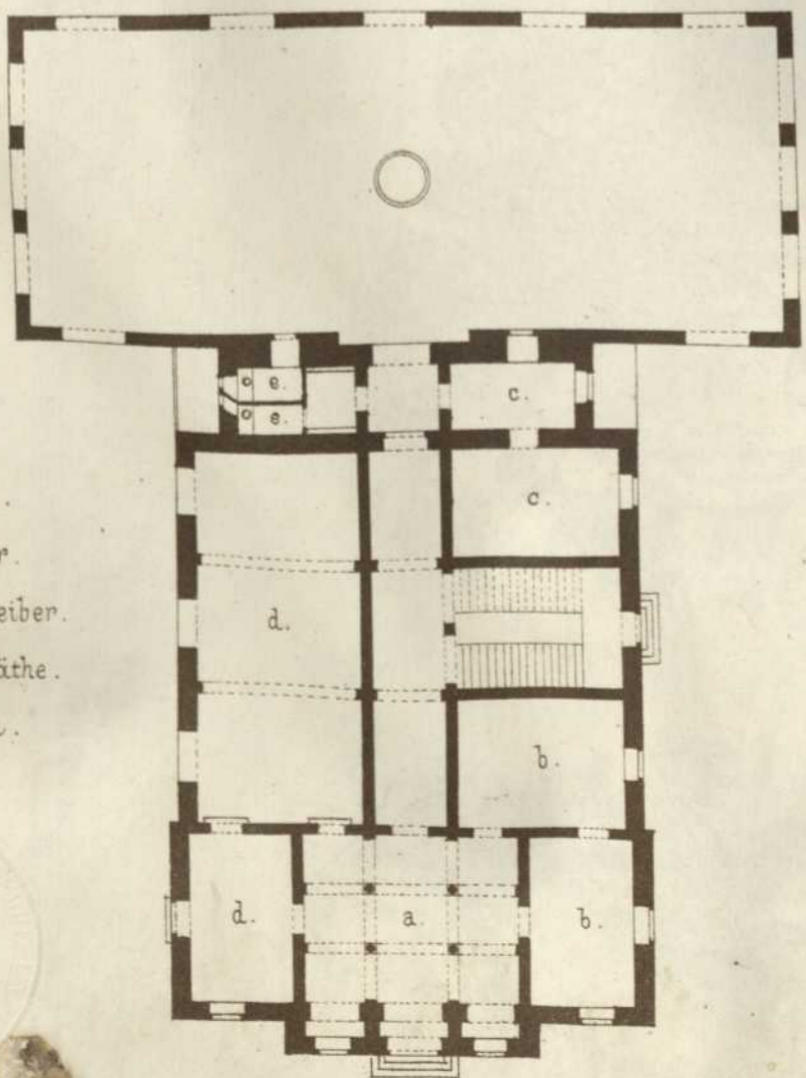
Erdgeschoss.
