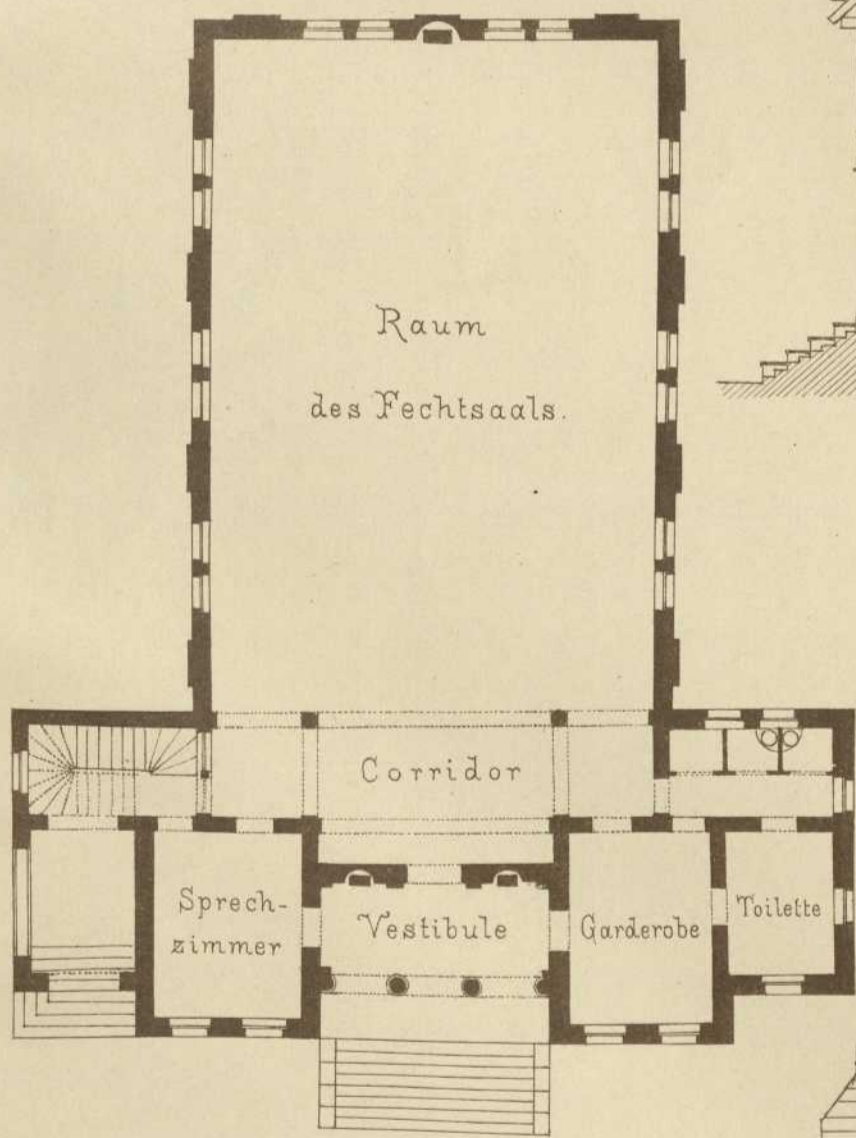
Erdgeschoss.
