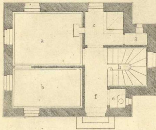
I. Stock.
