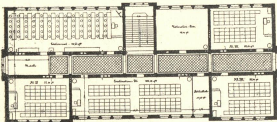
II. Obergeschoss.
