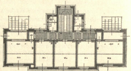
II. Obergeschoss.
