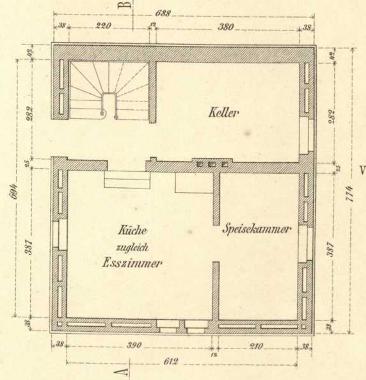
Erd-Geschoss.
