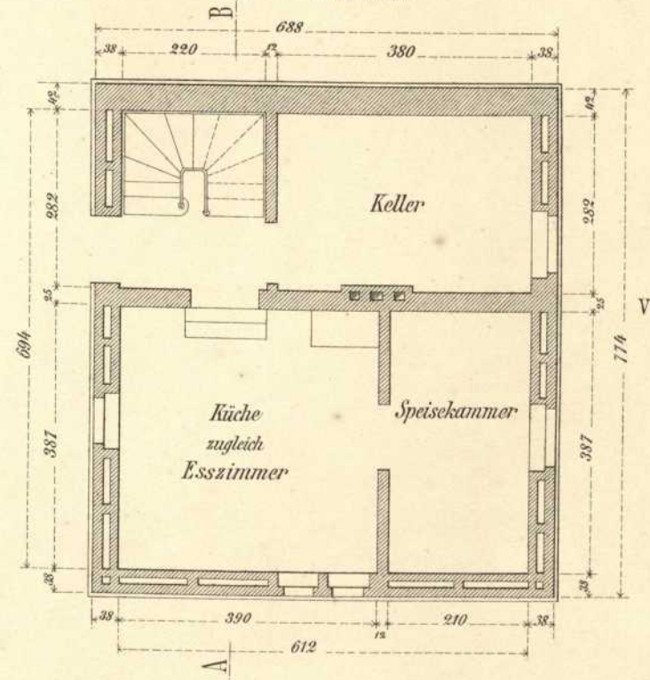
Erd-Geschoss.
