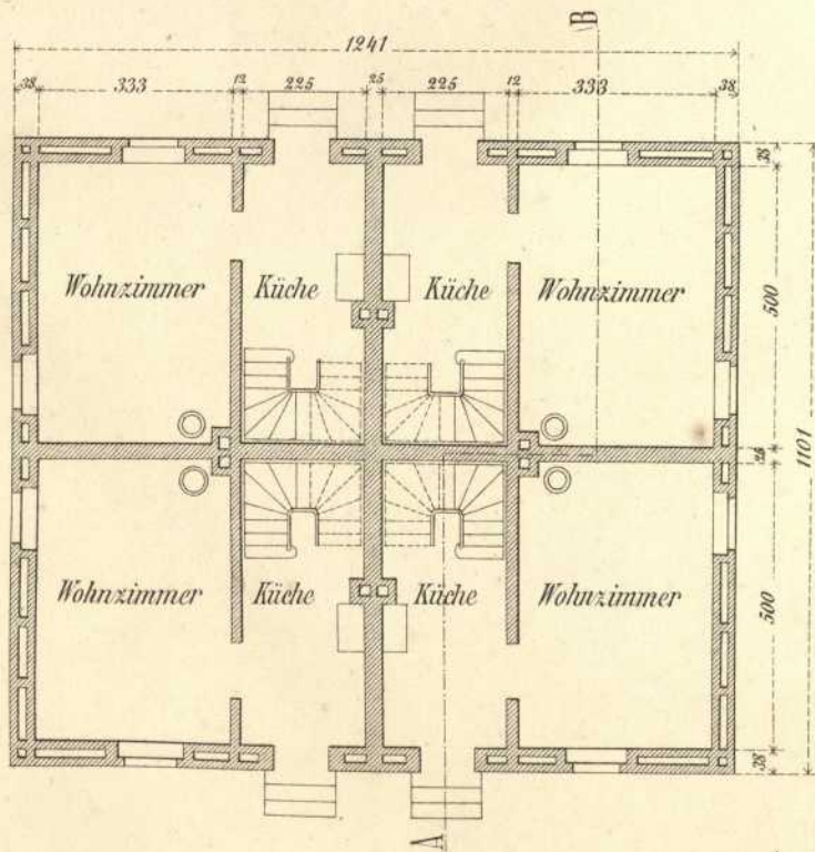
Erd-Geschoss.
