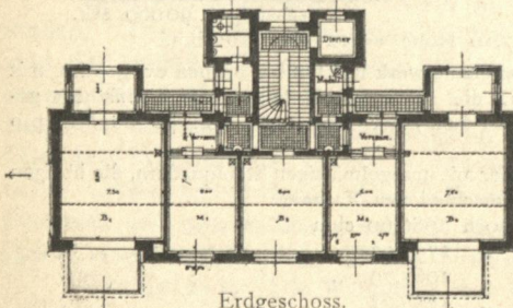
Erdgeschoss.
