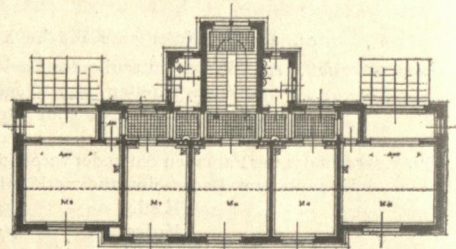
II. Obergeschoss.
